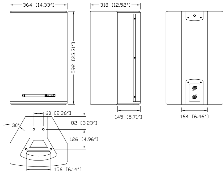
C6/C690 cabinet dimensions in mm [inch]
