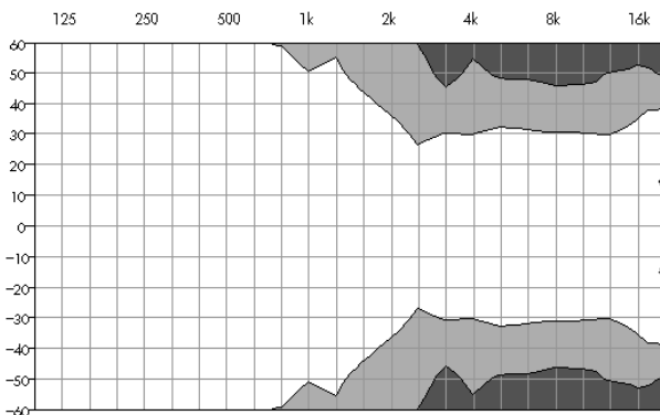
horizontal C6 isobar diagrams
