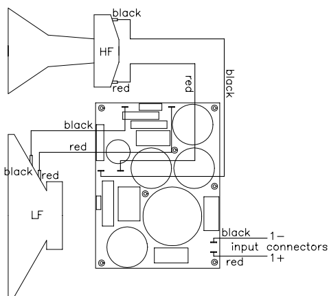
C6/C690 wiring diagram
