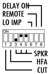
E-PAC Configuration for C6 (E-PAC version 2)
