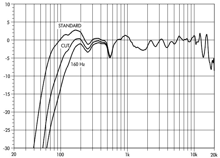
C6 frequency response, standard, CUT and 160 Hz switch settings
