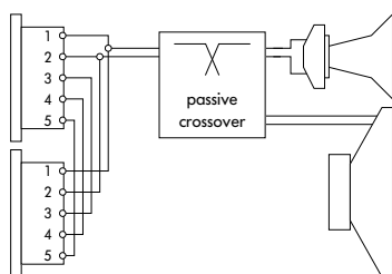
Connector wiring
