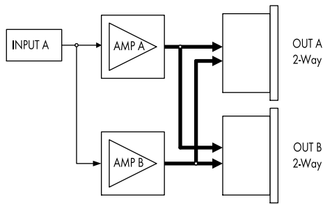
Input/Output routing "2-Way Active" *
